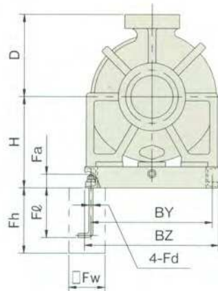
Flange (JIS10K or equivalent) Units: mm
