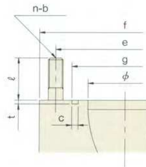
Flange (JIS10K or equivalent) Units: mm
