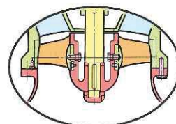
Adjustable Pitch Construction For B series Impeller
