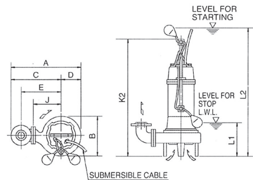
No.2 PUMP MODEL DLA
