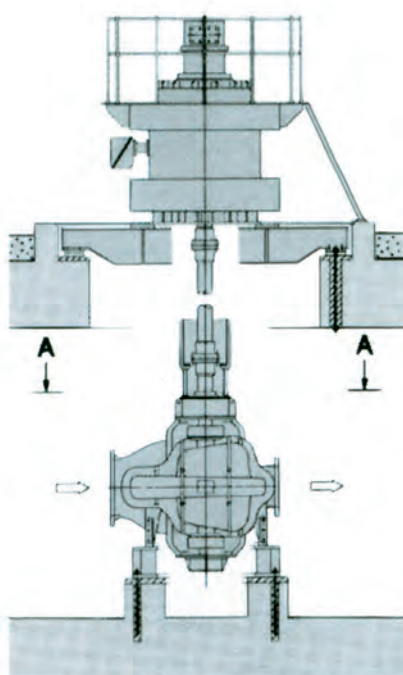
Two Floor Type
