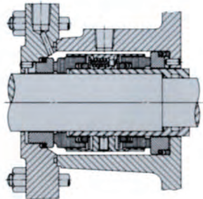
1C Double seal (Atmosphere side balance type)
