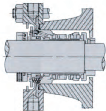
2B Knife edge Double seal
