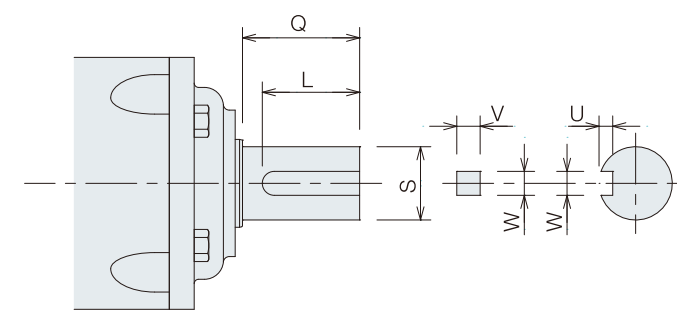
SHAFT
